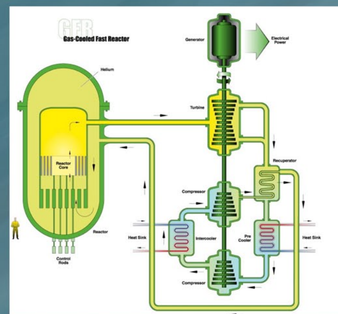
Gas Cooled
